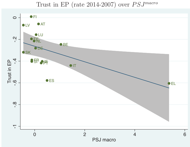
Figure 5. Trust in EP (rate 2014–2007) over PSJ^{macro}
